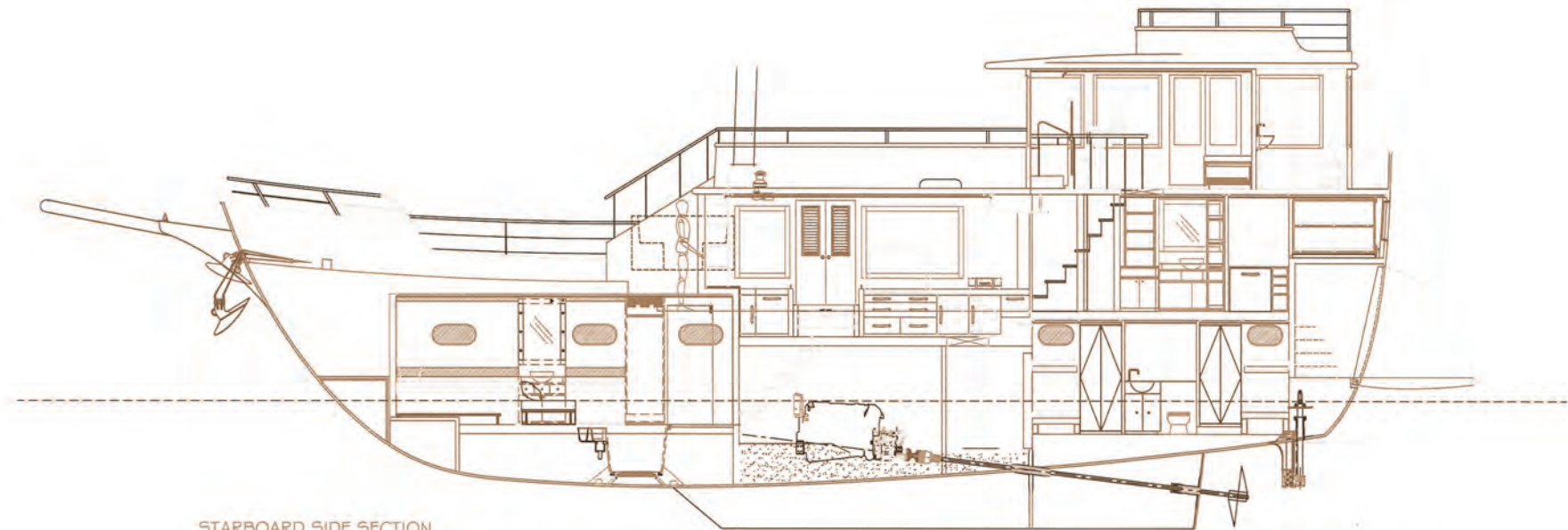
STARBOARD SIDE SECTION
