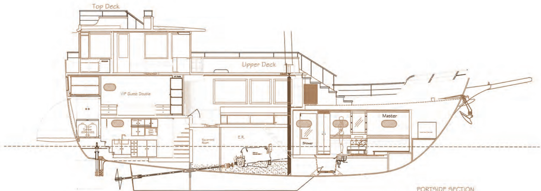
PORTSIDE SECTION
